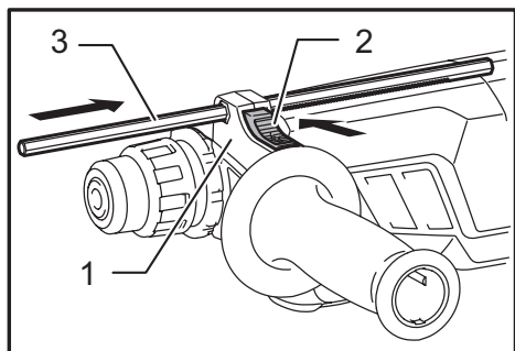
► 1. Grip base 2. Lock button 3. Depth gauge
